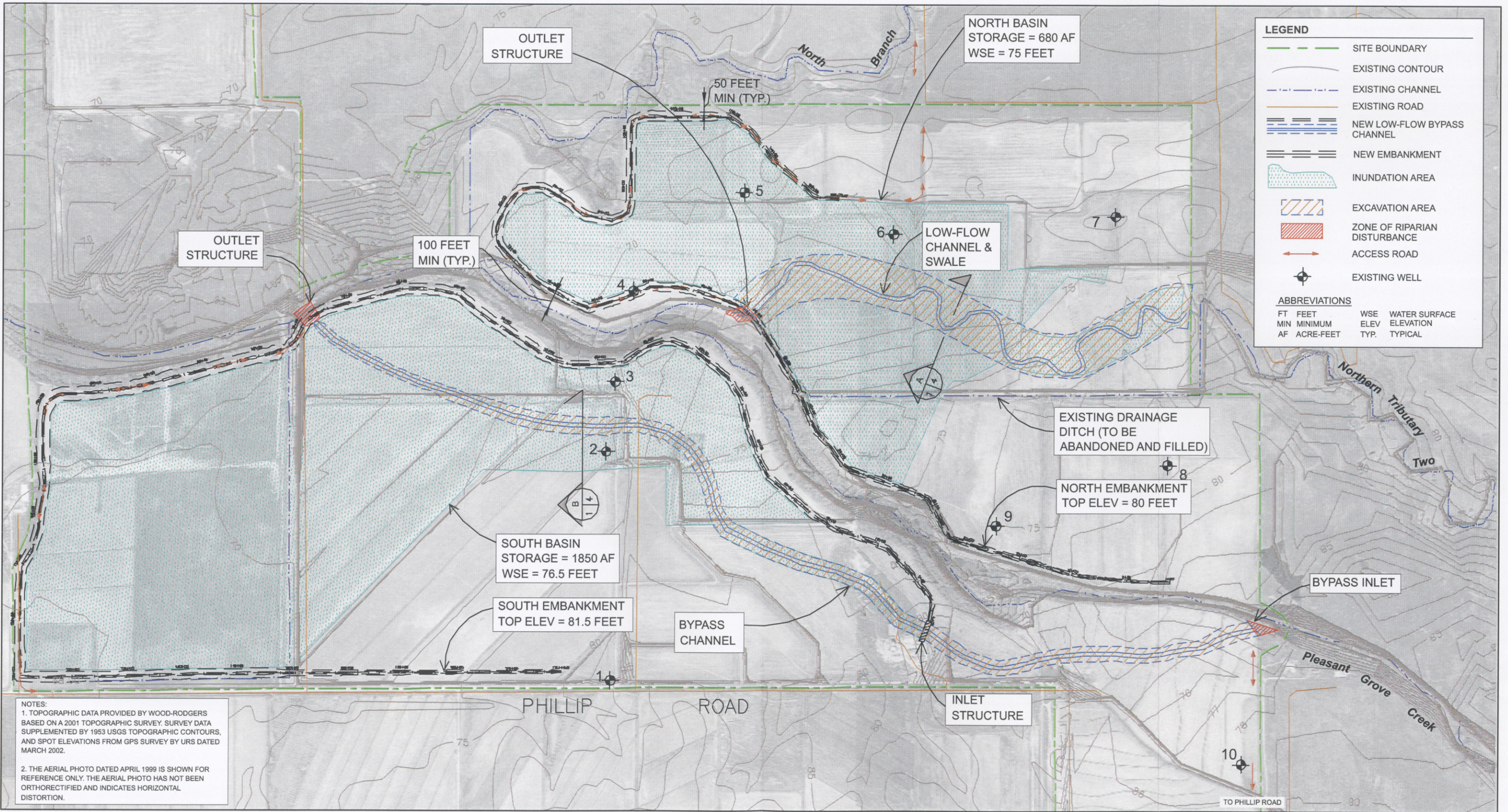
Figure 3 PLAN VIEW
